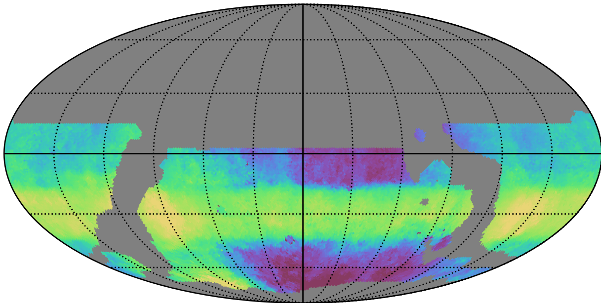
weather_cloudso8v3.4_10yrs WFD z band: Median HA
