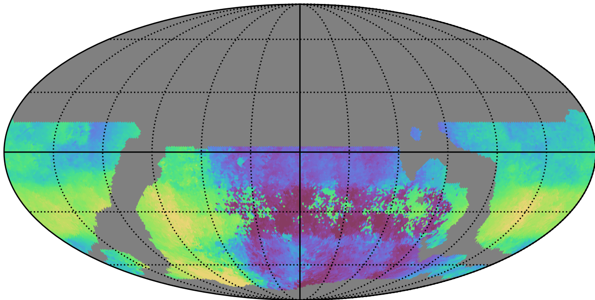
weather_cloudso8v3.4_10yrs WFD u band: Median HA
