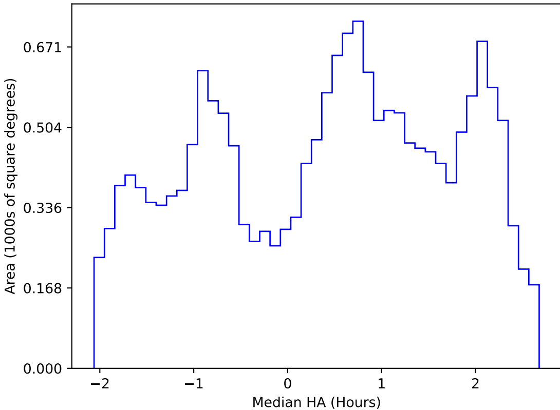
weather_cloudso8v3.4_10yrs WFD u band: Median HA
