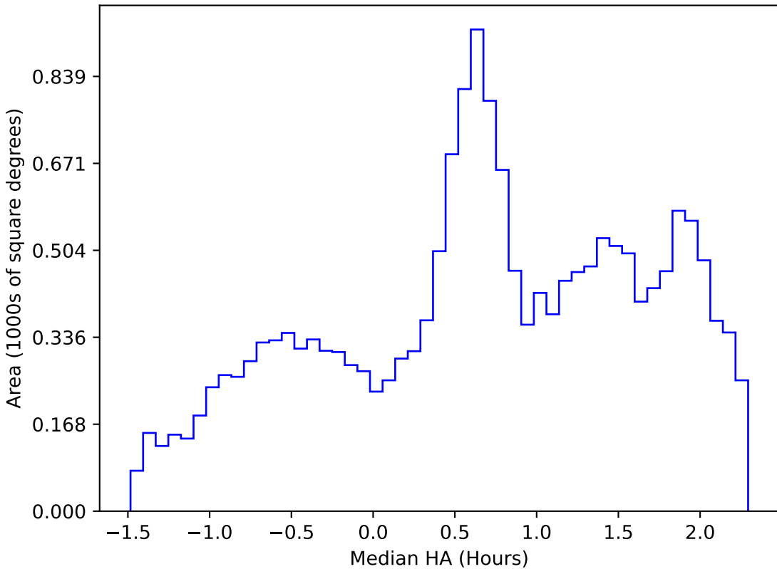
weather_cloudso8v3.4_10yrs WFD r band: Median HA
