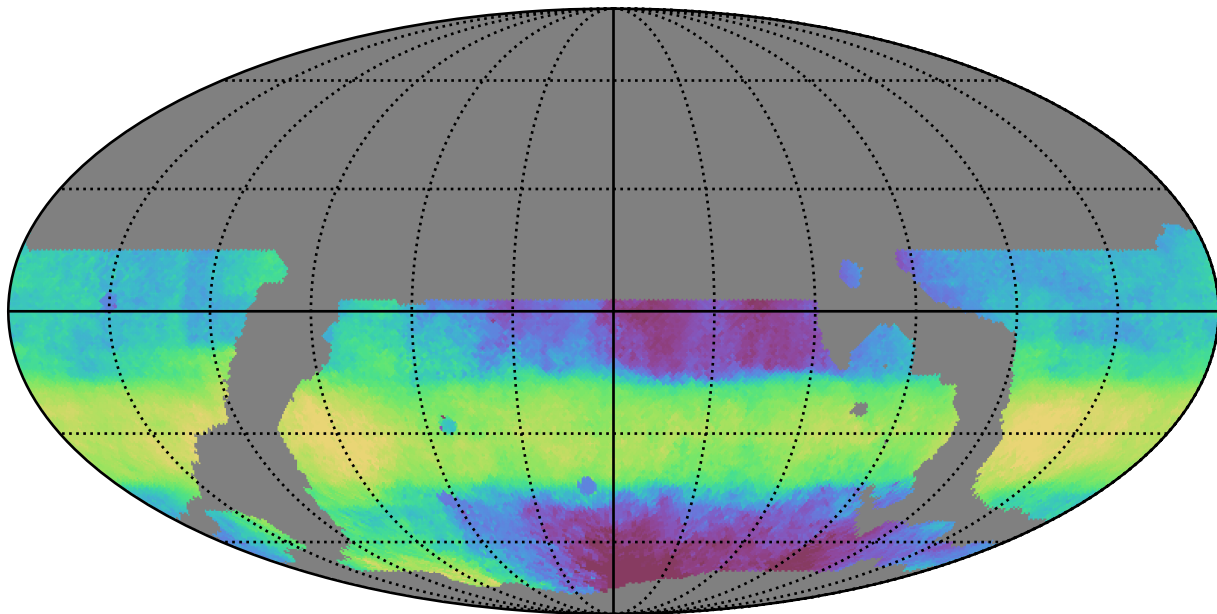
weather_cloudso8v3.4_10yrs WFD i band: Median HA
