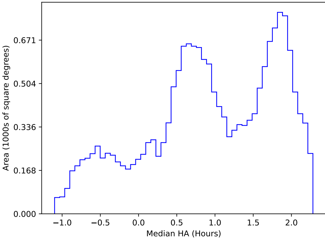
weather_cloudso8v3.4_10yrs WFD i band: Median HA
