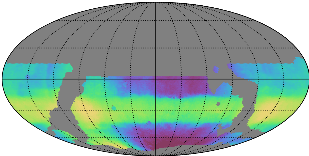
weather_cloudso8v3.4_10yrs WFD all bands: Median HA
