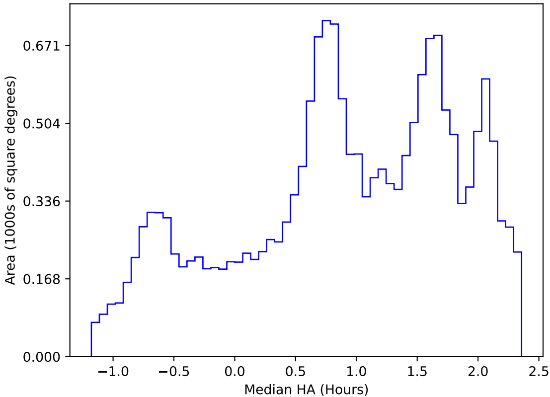
weather_cloudso8v3.4_10yrs WFD all bands: Median HA
