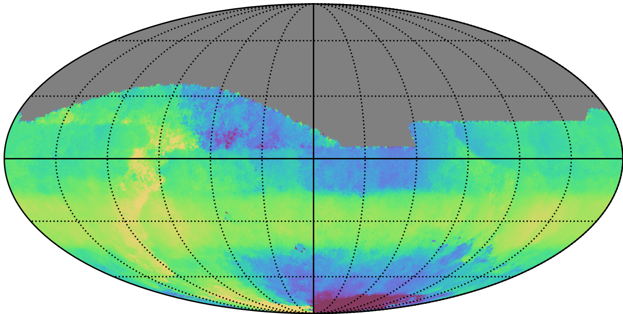
weather_cloudso8v3.4_10yrs All sky z band: Median HA
