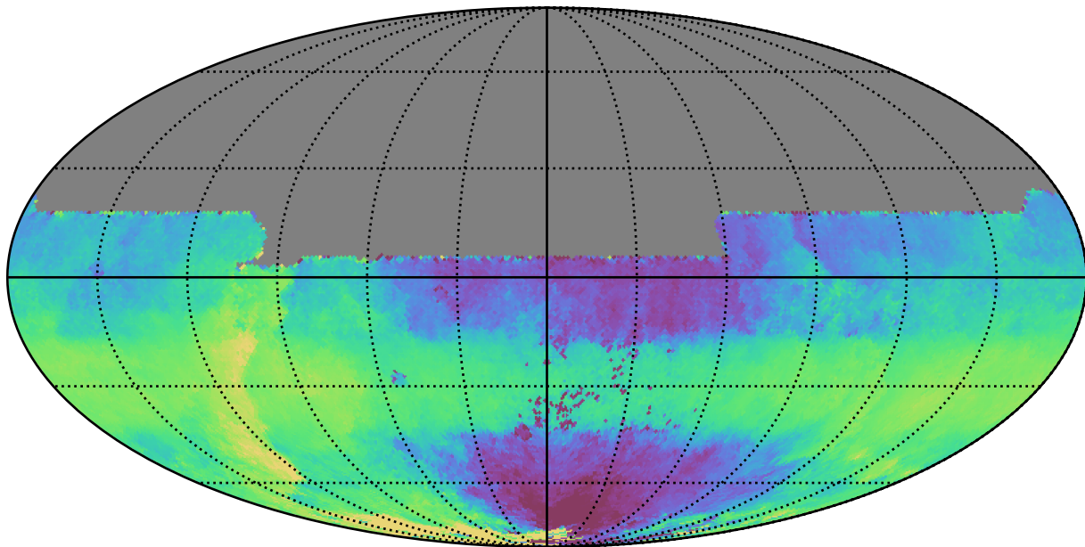
weather_cloudso8v3.4_10yrs All sky y band: Median HA
