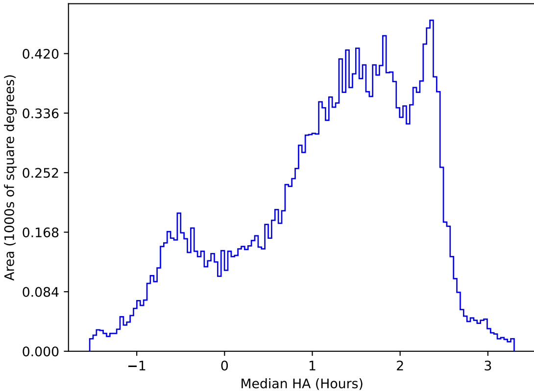
weather_cloudso8v3.4_10yrs All sky y band: Median HA
