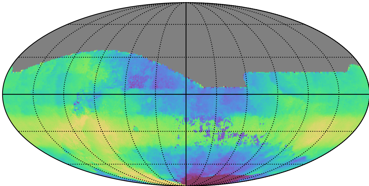
weather_cloudso8v3.4_10yrs All sky r band: Median HA
