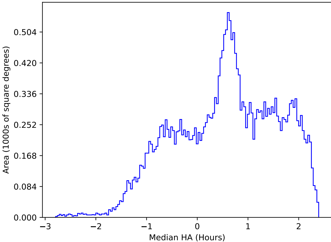
weather_cloudso8v3.4_10yrs All sky r band: Median HA
