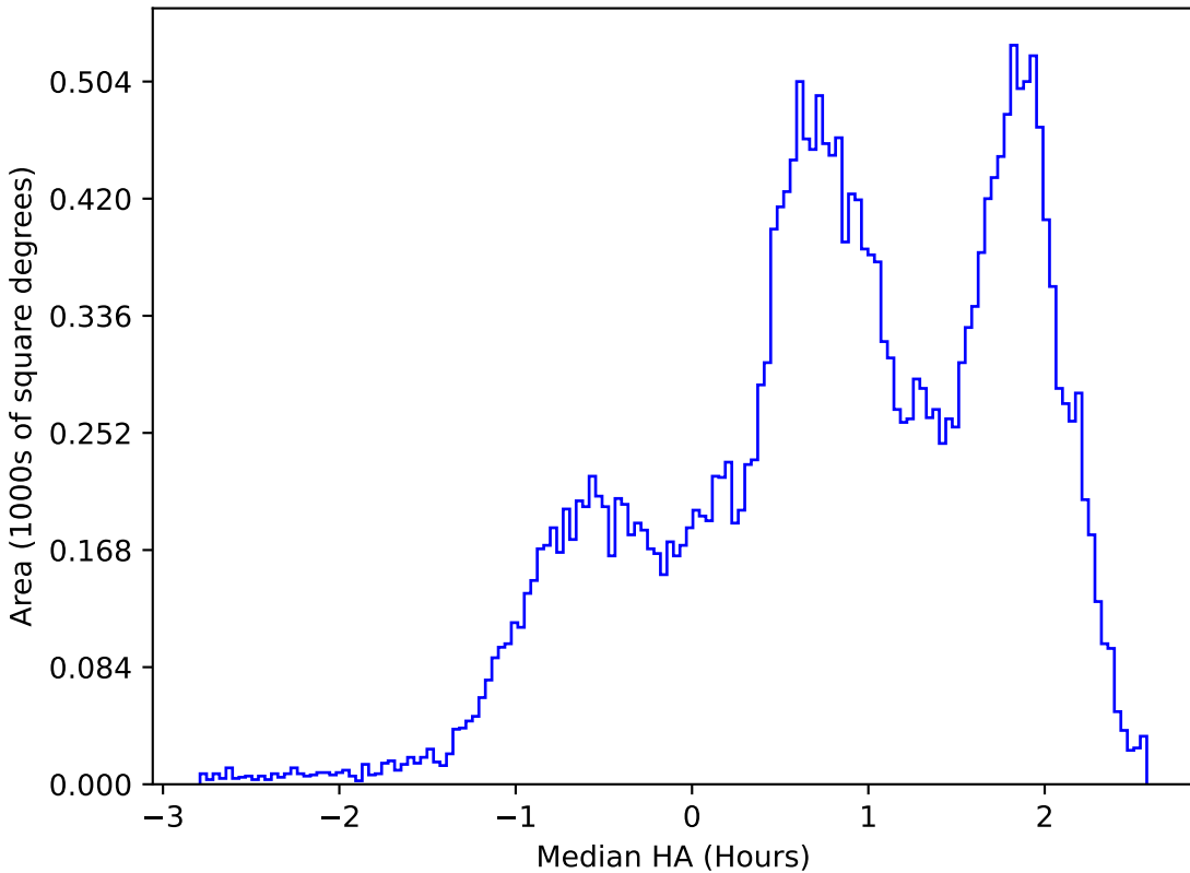
weather_cloudso8v3.4_10yrs All sky i band: Median HA
