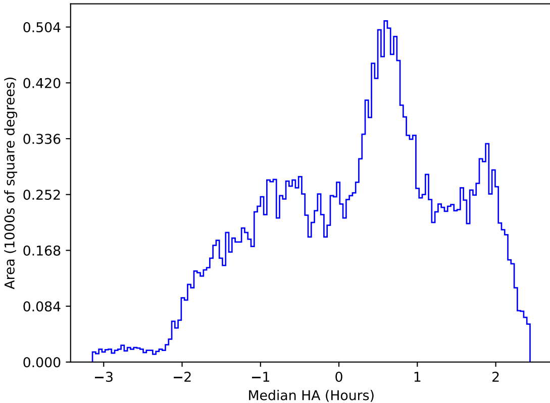
weather_cloudso8v3.4_10yrs All sky g band: Median HA
