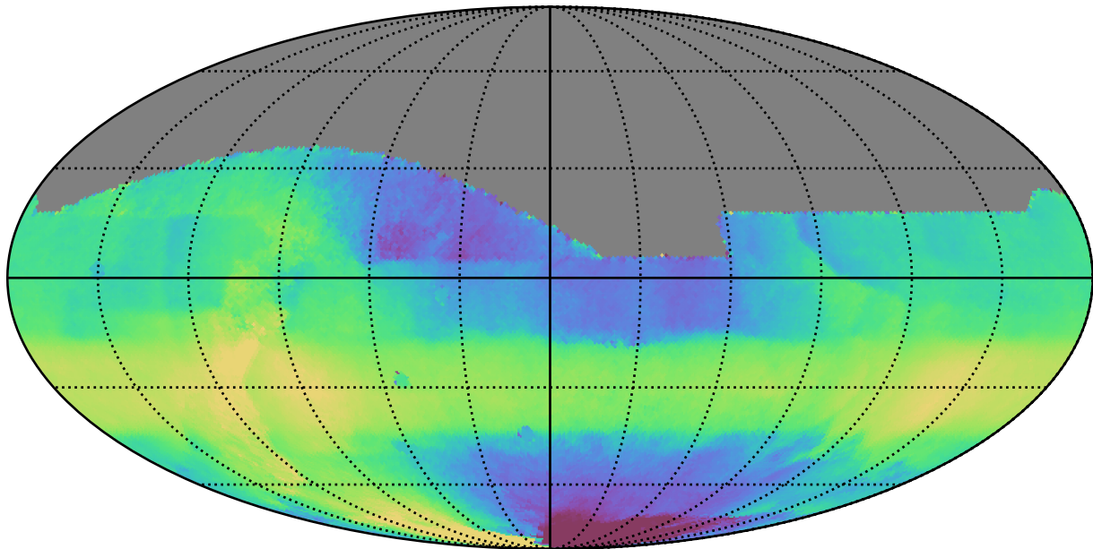
weather_cloudso8v3.4_10yrs All sky all bands: Median HA
