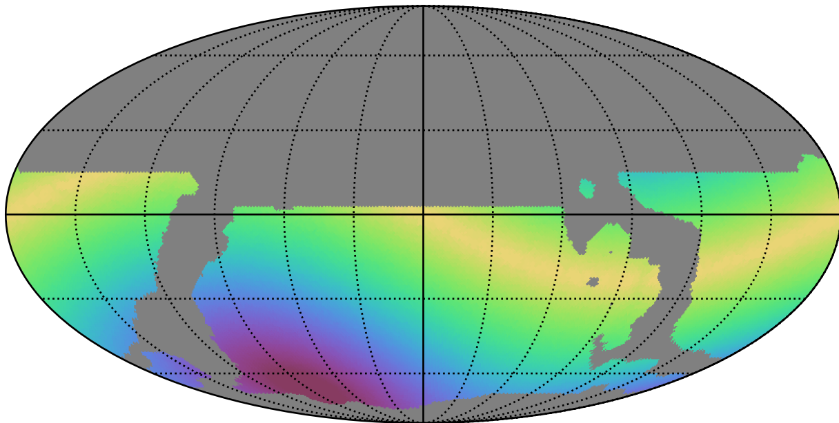
weather_cloudso8v3.4_10yrs WFD z band: Max solarElong
