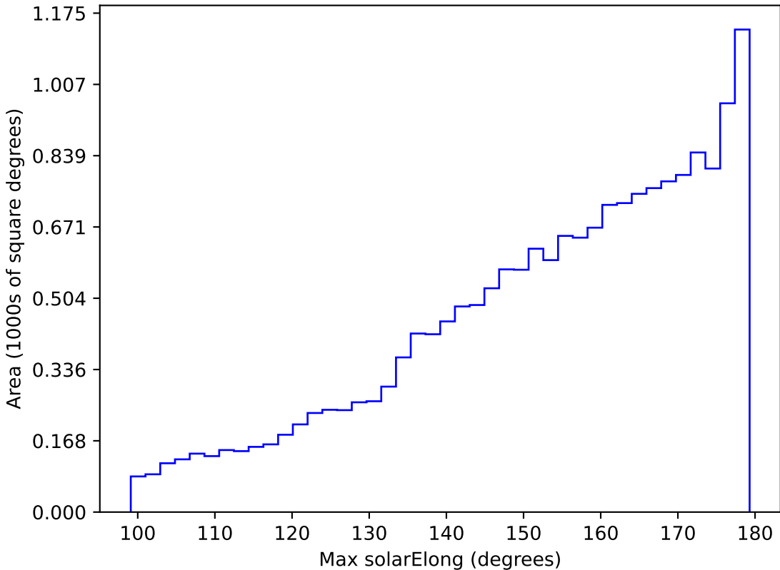
weather_cloudso8v3.4_10yrs WFD z band: Max solarElong
