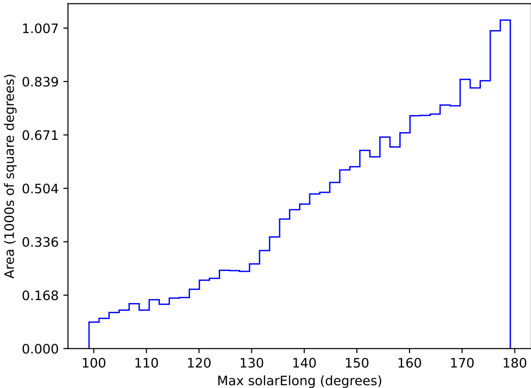
weather_cloudso8v3.4_10yrs WFD y band: Max solarElong
