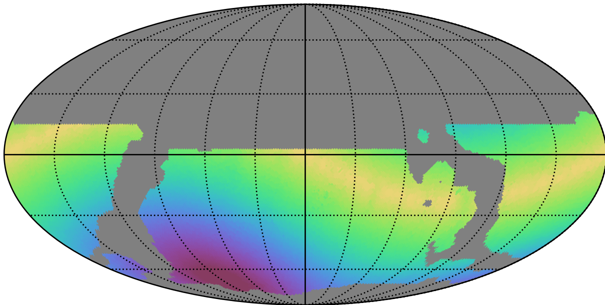
weather_cloudso8v3.4_10yrs WFD u band: Max solarElong
