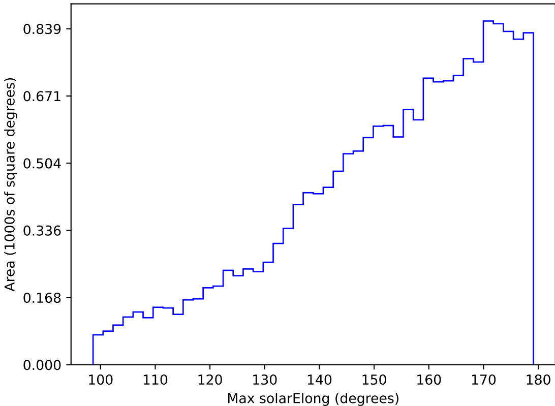
weather_cloudso8v3.4_10yrs WFD u band: Max solarElong
