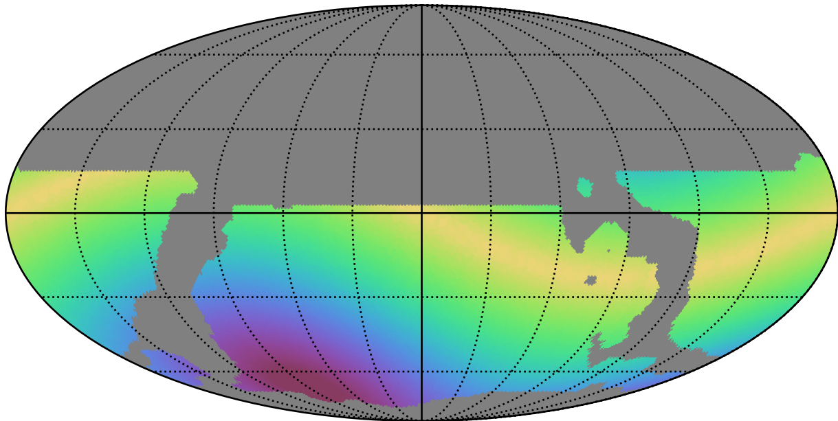
weather_cloudso8v3.4_10yrs WFD r band: Max solarElong
