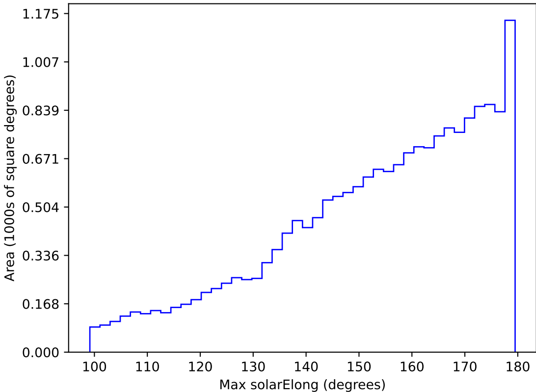
weather_cloudso8v3.4_10yrs WFD r band: Max solarElong
