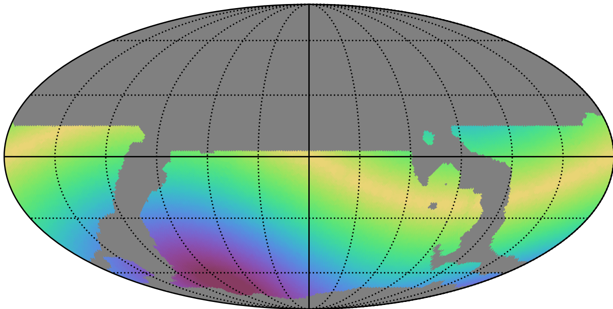
weather_cloudso8v3.4_10yrs WFD i band: Max solarElong
