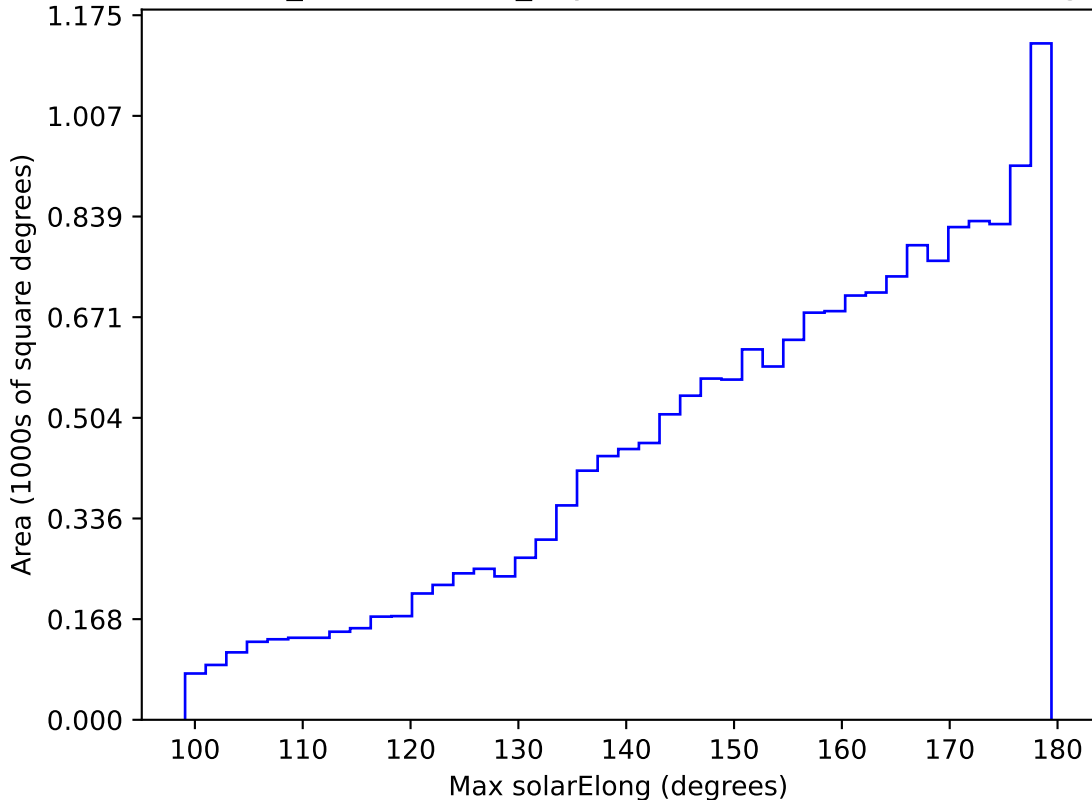
weather_cloudso8v3.4_10yrs WFD i band: Max solarElong
