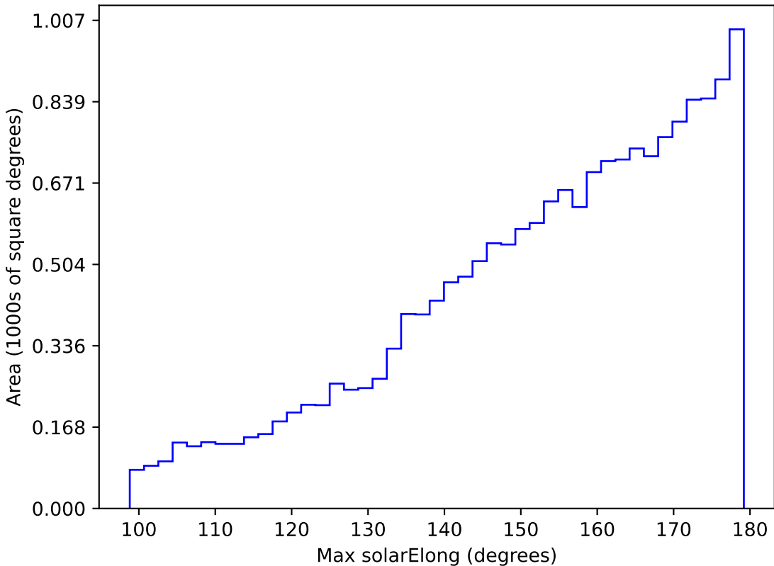
weather_cloudso8v3.4_10yrs WFD g band: Max solarElong
