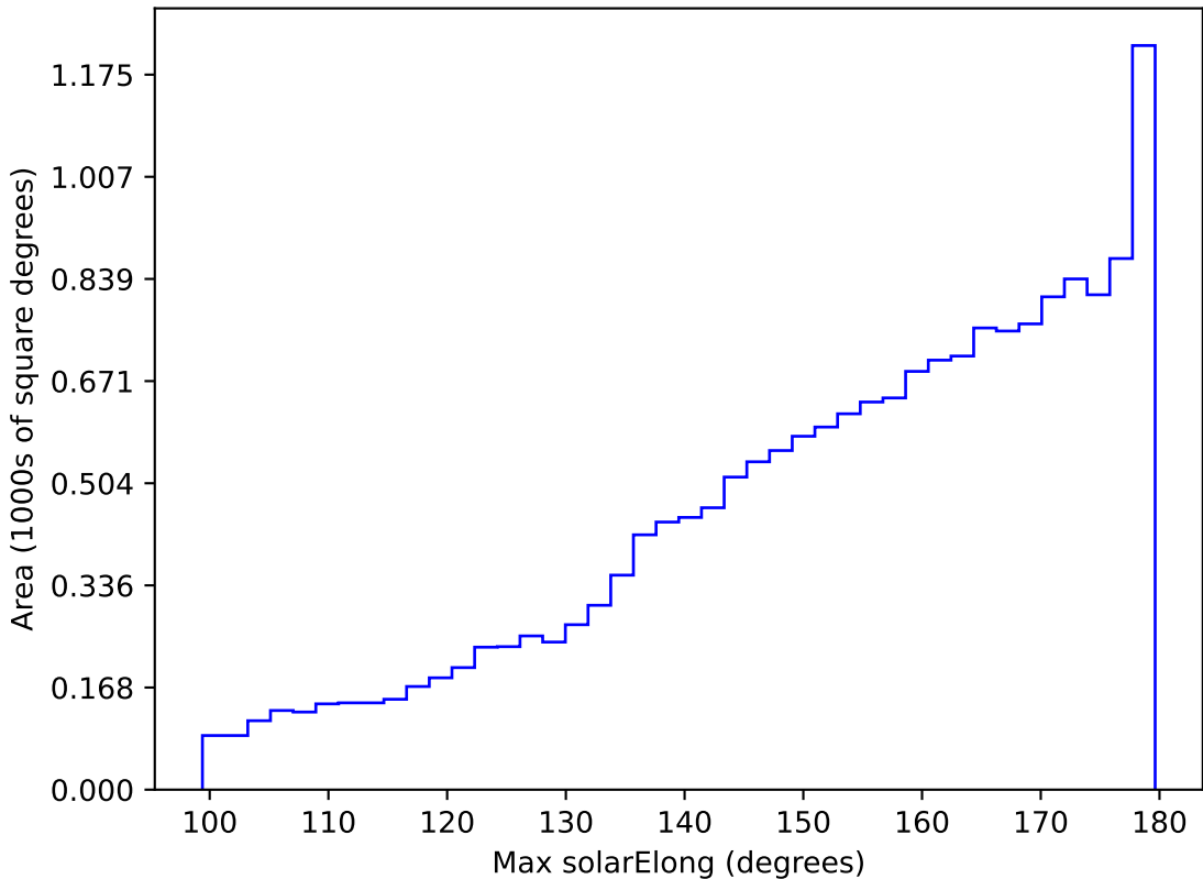
weather_cloudso8v3.4_10yrs WFD all bands: Max solarElong
