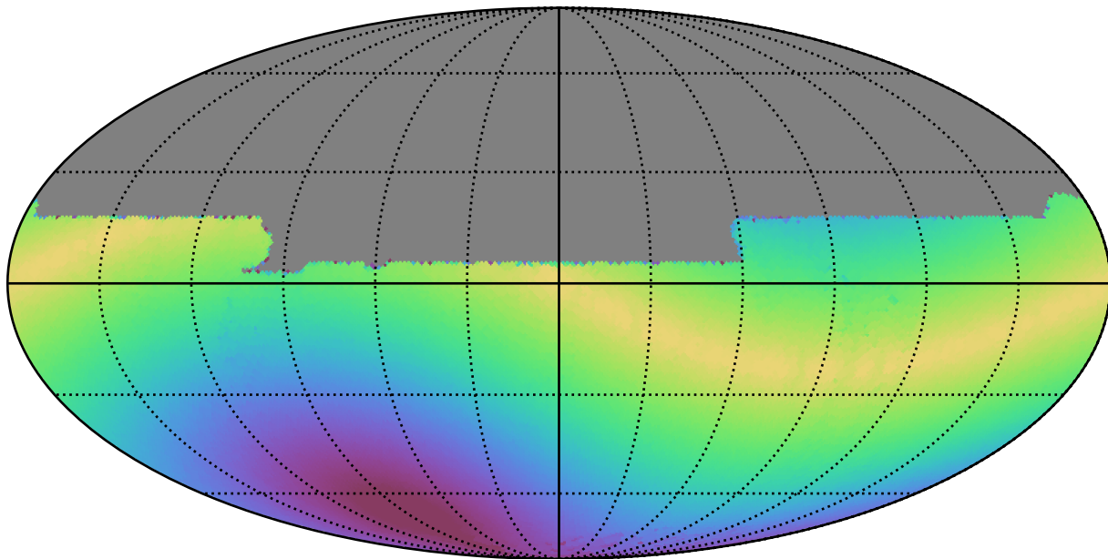
weather_cloudso8v3.4_10yrs All sky y band: Max solarElong
