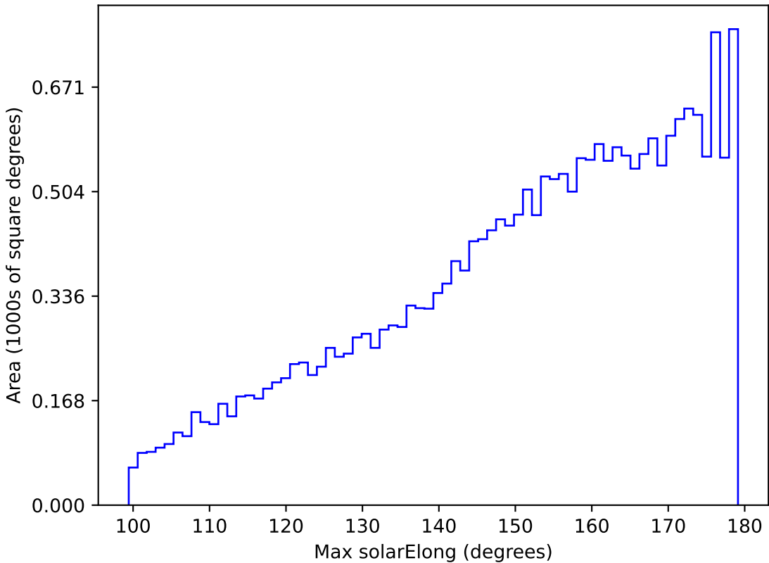
weather_cloudso8v3.4_10yrs All sky y band: Max solarElong
