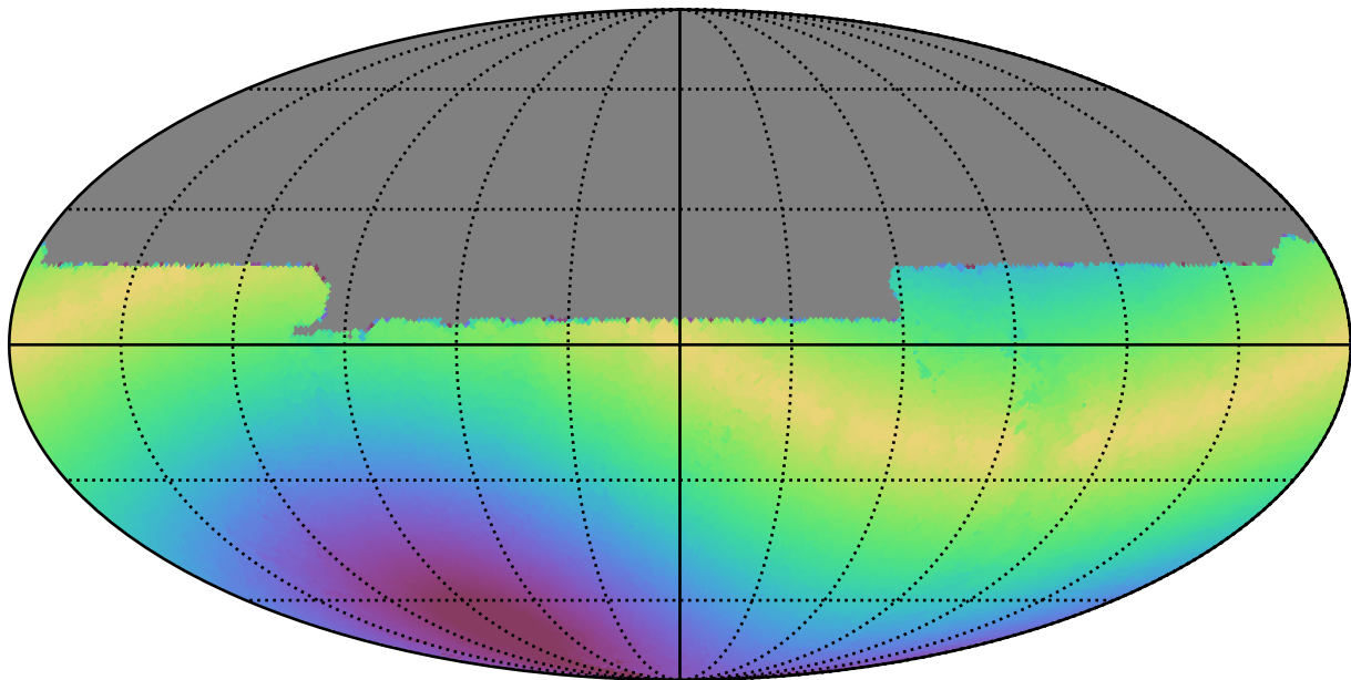
weather_cloudso8v3.4_10yrs All sky u band: Max solarElong
