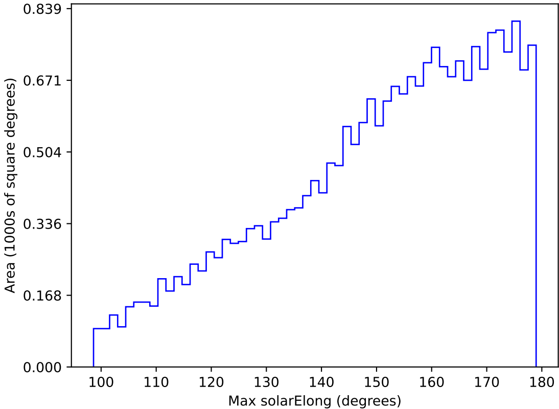
weather_cloudso8v3.4_10yrs All sky u band: Max solarElong
