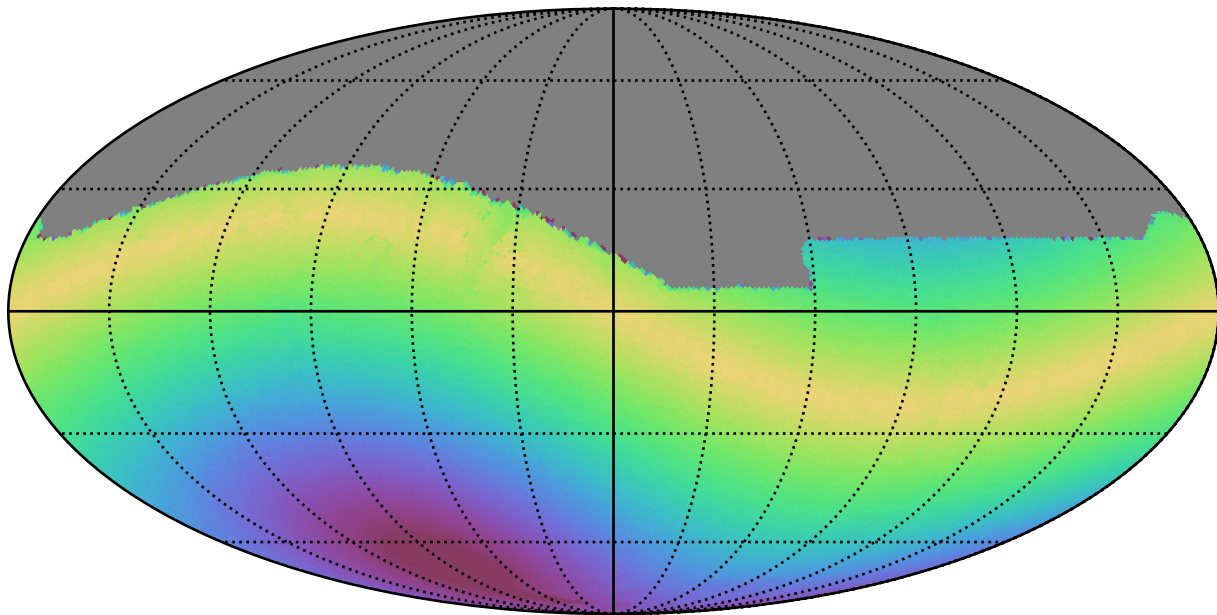
weather_cloudso8v3.4_10yrs All sky r band: Max solarElong
