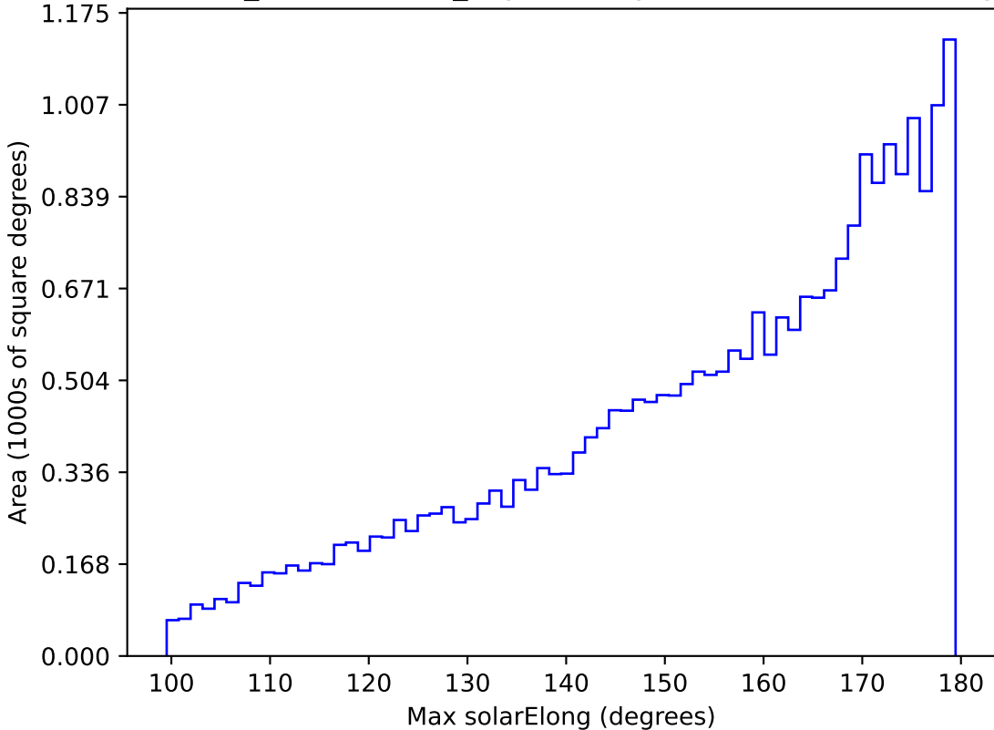
weather_cloudso8v3.4_10yrs All sky r band: Max solarElong
