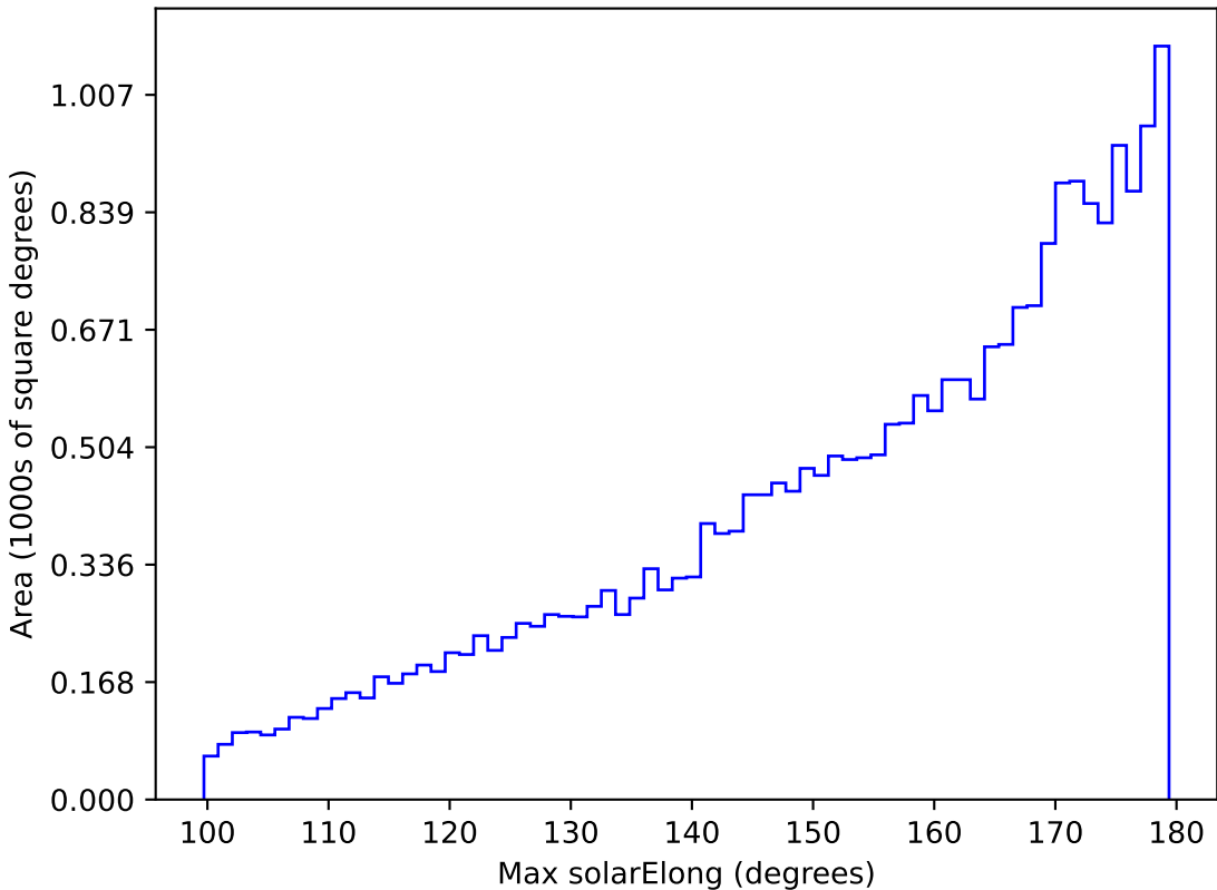
weather_cloudso8v3.4_10yrs All sky i band: Max solarElong
