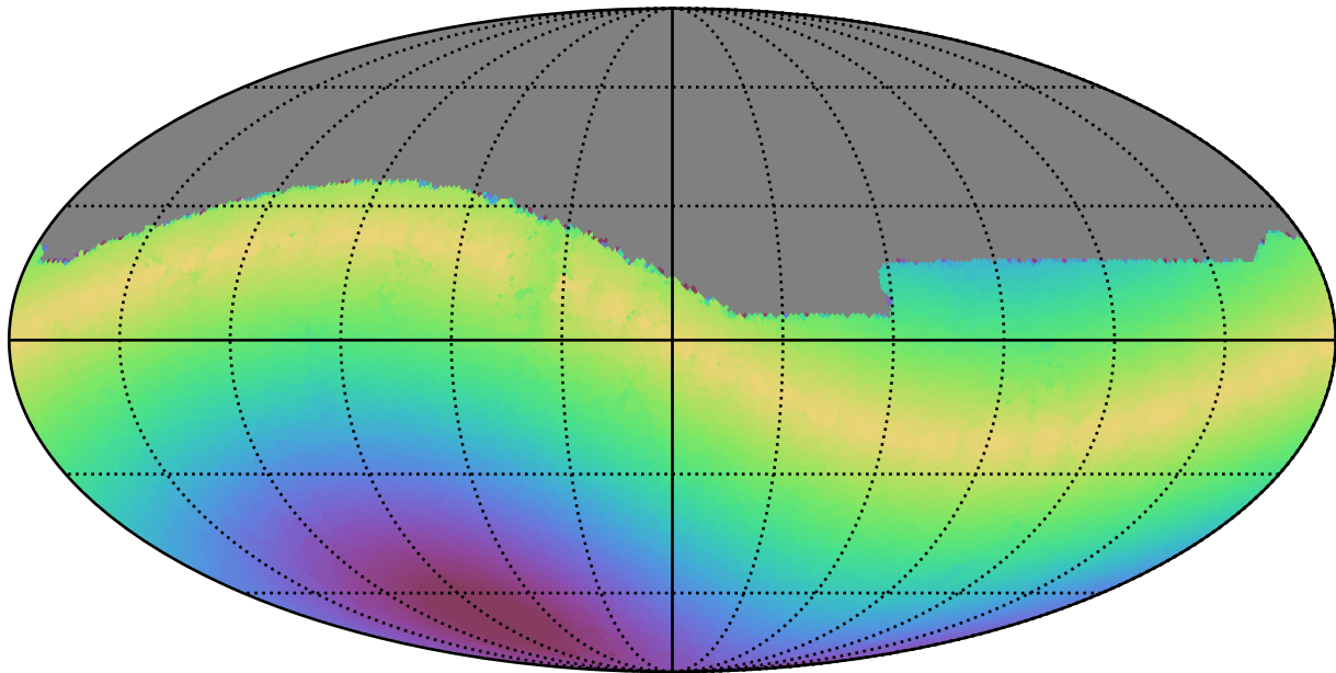
weather_cloudso8v3.4_10yrs All sky g band: Max solarElong
