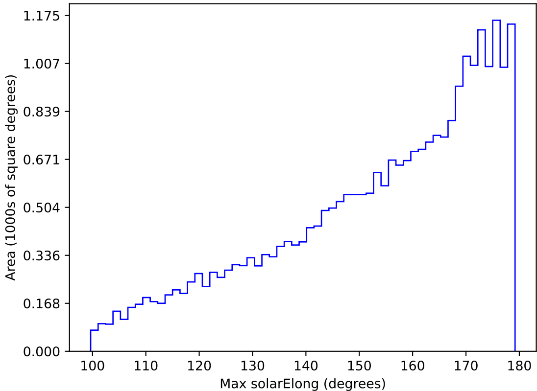
weather_cloudso8v3.4_10yrs All sky g band: Max solarElong
