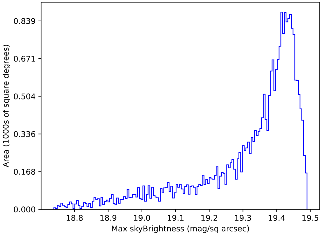
weather_cloudso8v3.4_10yrs Yr 1 z band: Max skyBrightness
