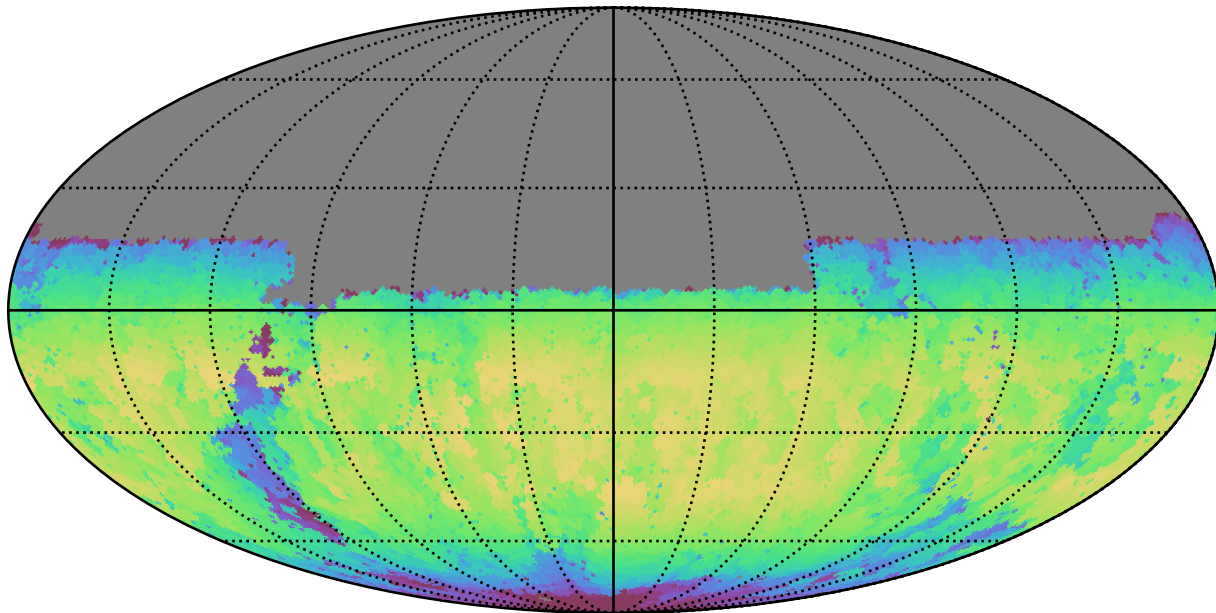
weather_cloudso8v3.4_10yrs Yr 1 y band: Max skyBrightness
