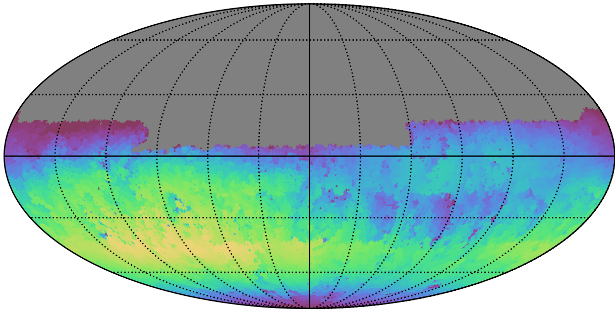
weather_cloudso8v3.4_10yrs Yr 1 u band: Max skyBrightness
