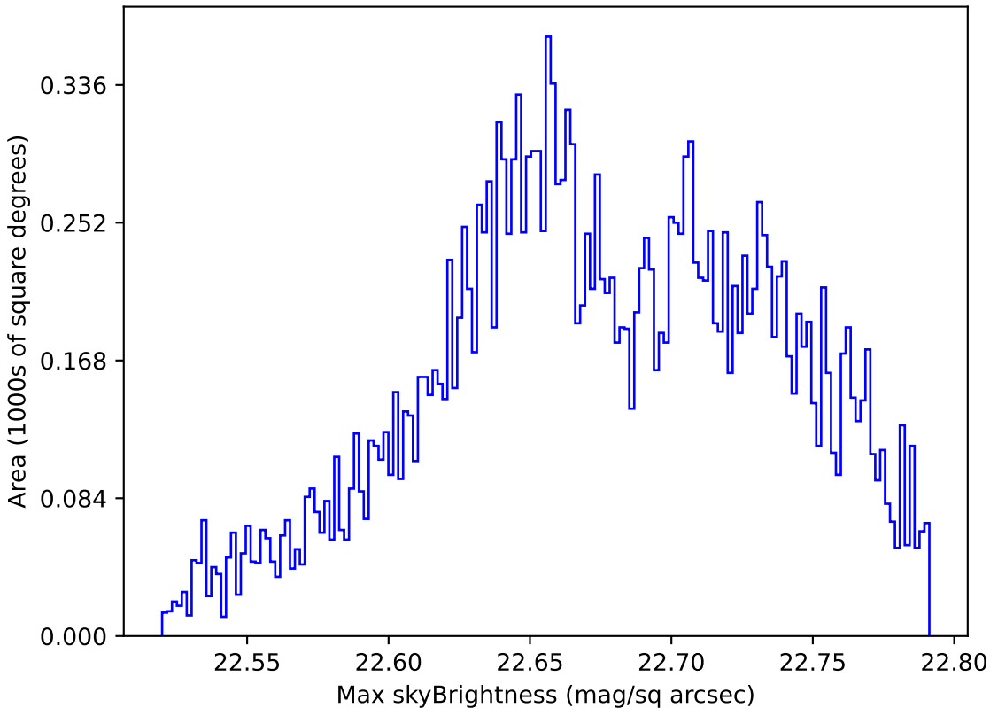
weather_cloudso8v3.4_10yrs Yr 1 u band: Max skyBrightness
