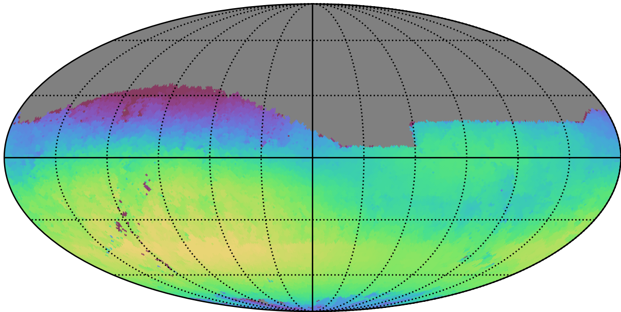
weather_cloudso8v3.4_10yrs Yr 1 r band: Max skyBrightness
