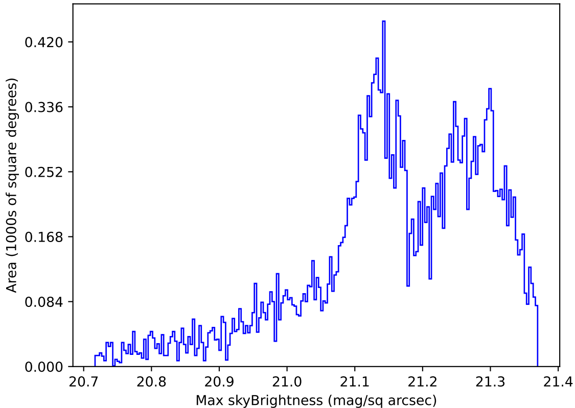
weather_cloudso8v3.4_10yrs Yr 1 r band: Max skyBrightness
