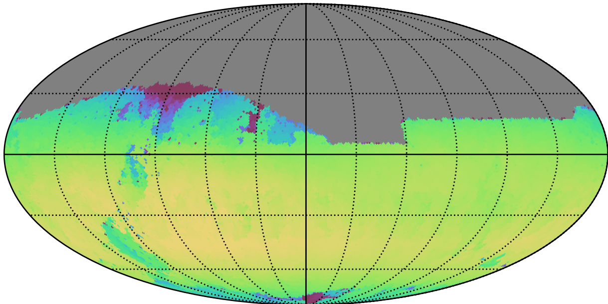
weather_cloudso8v3.4_10yrs Yr 1 i band: Max skyBrightness
