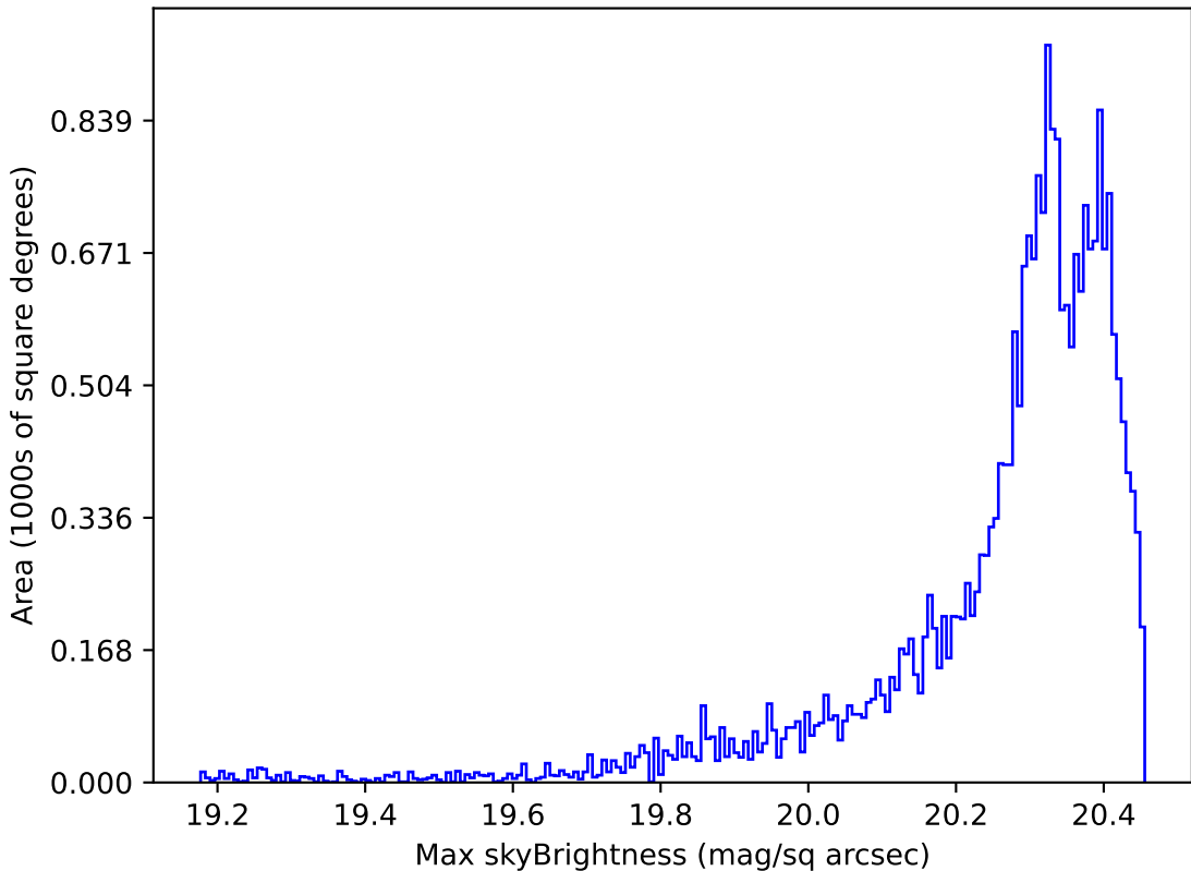
weather_cloudso8v3.4_10yrs Yr 1 i band: Max skyBrightness
