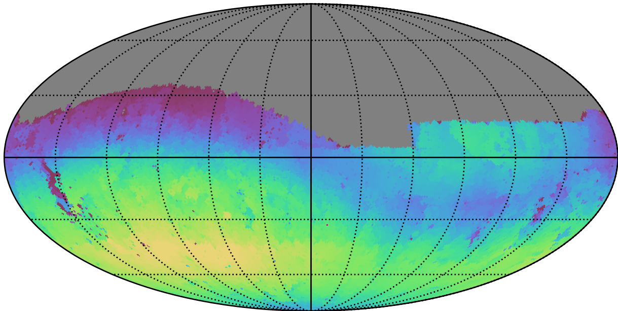
weather_cloudso8v3.4_10yrs Yr 1 g band: Max skyBrightness
