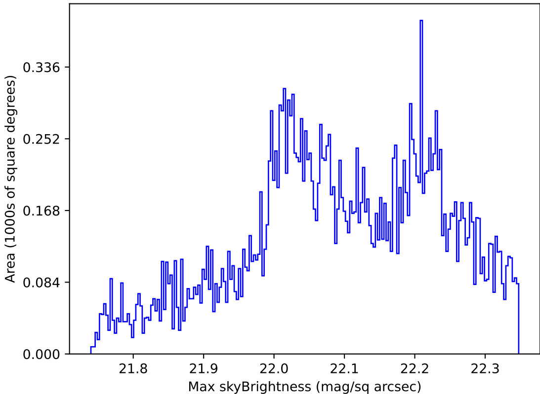
weather_cloudso8v3.4_10yrs Yr 1 g band: Max skyBrightness
