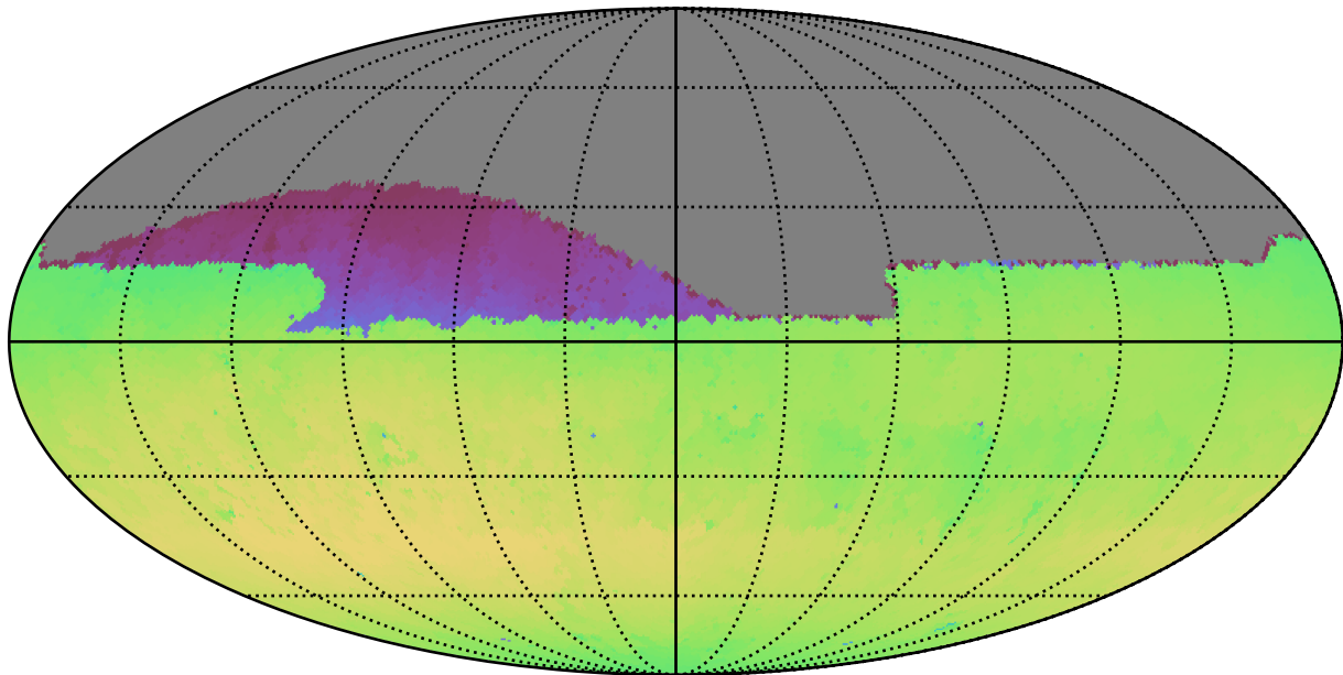
weather_cloudso8v3.4_10yrs Yr1 all bands: Max skyBrightness
