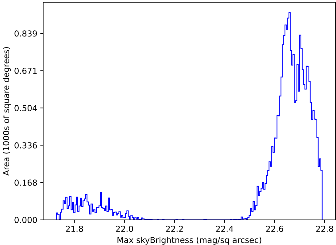
weather_cloudso8v3.4_10yrs Yr 1 all bands: Max skyBrightness
