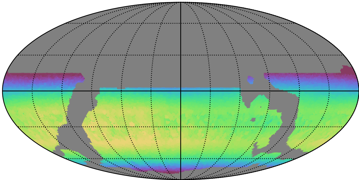
weather_cloudso8v3.4_10yrs WFD z band: Max skyBrightness
