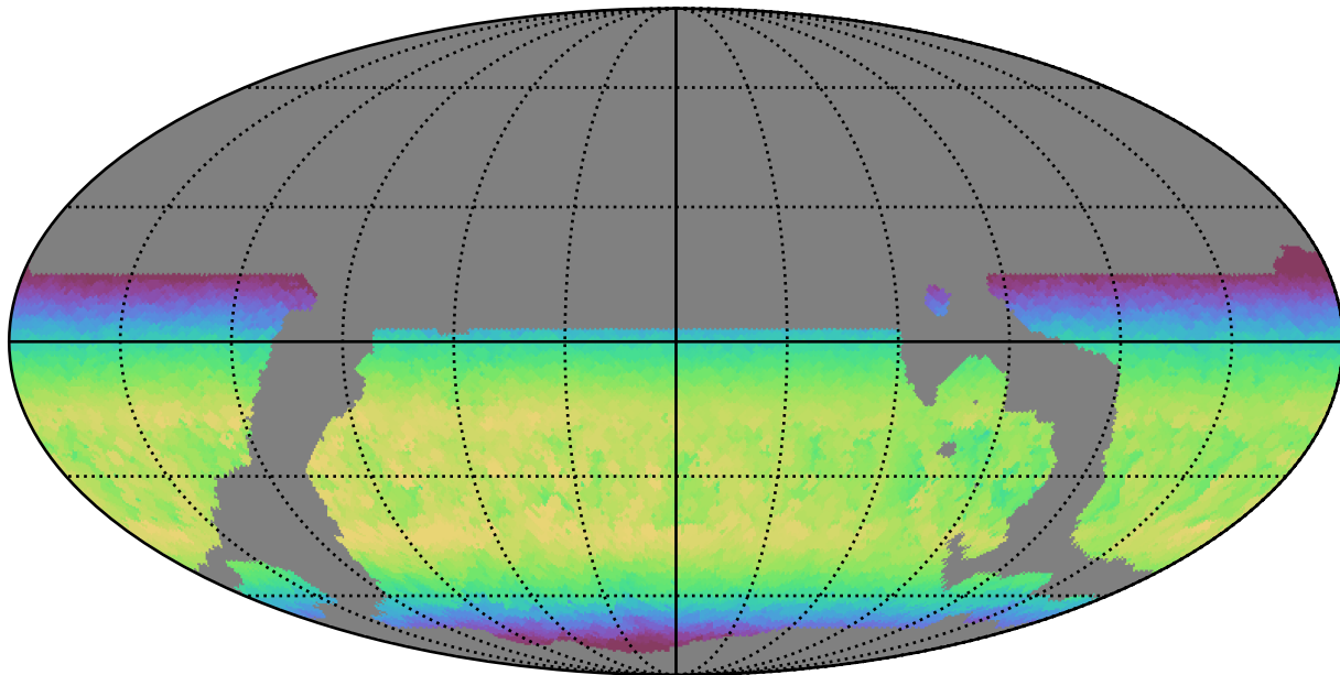
weather_cloudso8v3.4_10yrs WFD y band: Max skyBrightness
